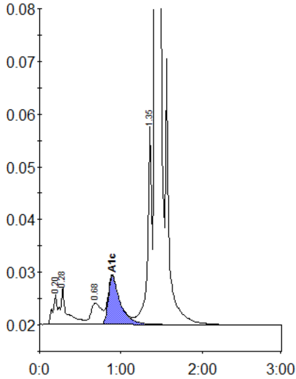
Peak table - ID: 10303266
